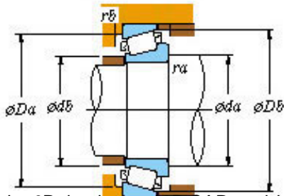
39585/20 Bearing 2D drawings and 3D CAD models
